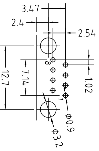
SUGGESTED PCB LAYOUT (TOP VIEW)
