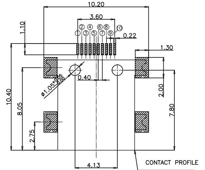
RECOMMENDED PCB LAYOUT(TOP VIEW) GENERAL TOLERANCES: ±0.05
