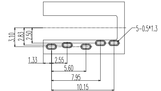
P.C.B LAYOUT (All SIZES±0.05mm) TOP VIEW
